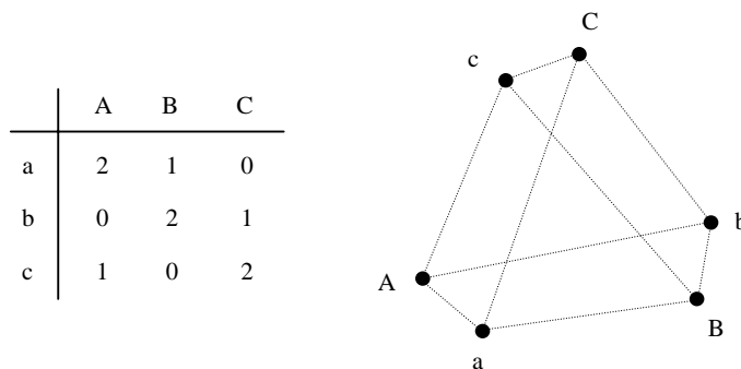
Figure 3: Spatial representation of cyclic preferences
