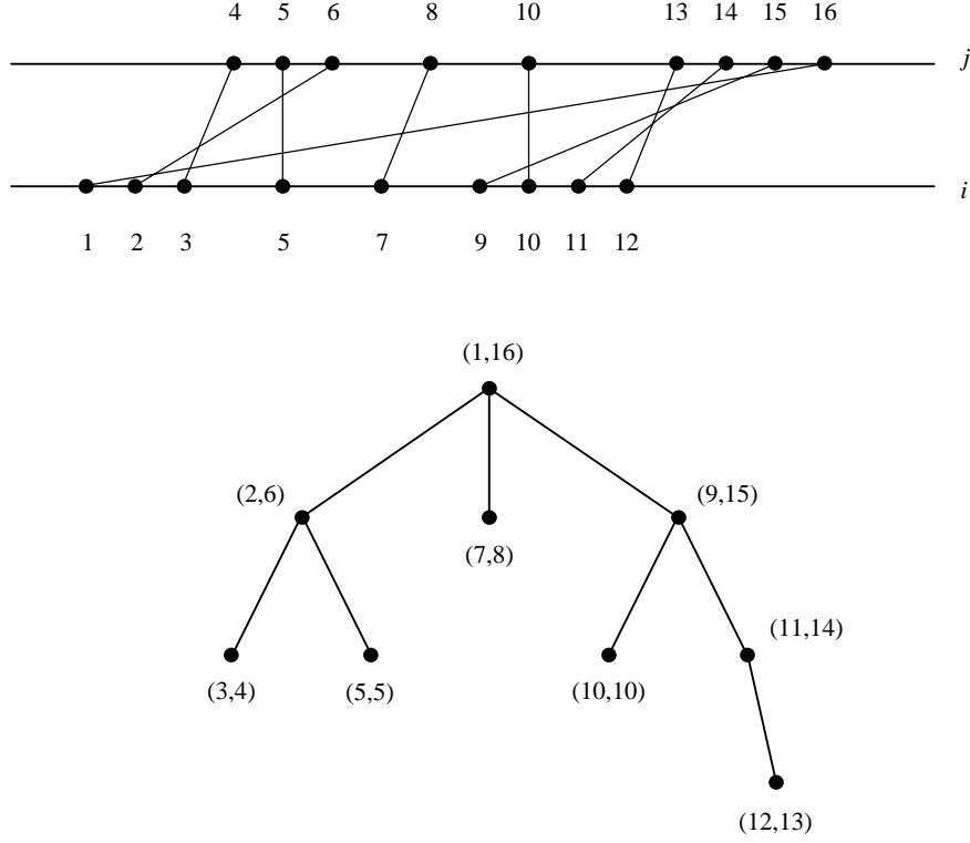
Figure 2: Tree structure of a nested cluster
