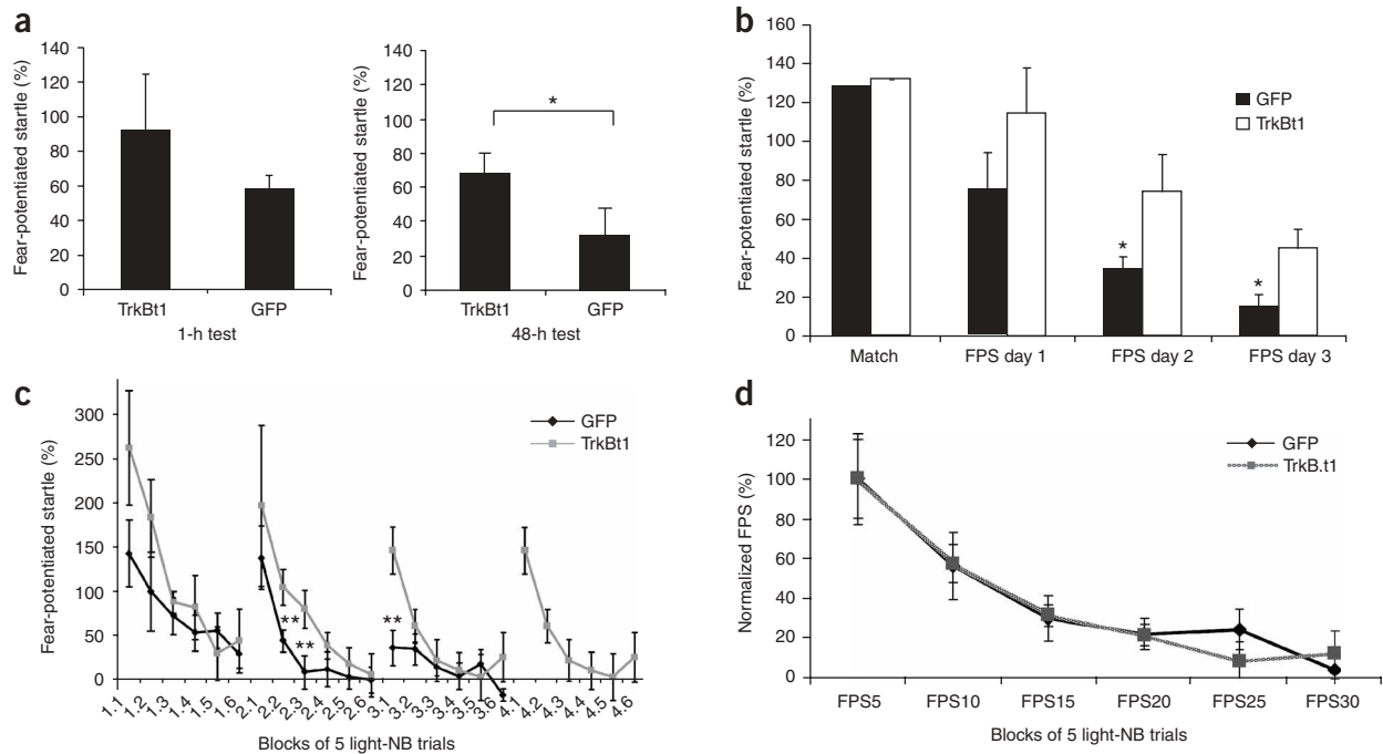
Figure 2 Lentivirus expression of TrkB.t1 in BLA blocks the consolidation but not the acquisition of extinction. (a) Level of fear-potentiated startle (FPS) following extinction training, when tested at 1 h or 48 h. TrkB.t1-infected rats showed significantly higher levels of fear 2 d after extinction, as compared to GFP-infected rats ( n = 9 and 7 for TrkB.t1 and GFP groups, respectively). (b) TrkB.t1 impairs extinction retention. Averaging across all trials, TrkB.t1-infected rats showed a deficit in extinction as compared to GFP-infected rats. (c) Examining extinction within the testing session suggested that the TrkB.t1-infected rats had normal within-session extinction, but lacked extinction retention across the 2-d interval between tests ( n = 9 and 10 for TrkB.t1 and GFP groups, respectively). Note that GFP-infected rats showed complete extinction by test 3 and were not tested thereafter. TrkB.t1-infected rats showed poor extinction retention even on day 4, as evidenced by high FPS during the first 5 trials of the test. (d) Normalization of FPS across the first 3 d (100% = mean of first 5 trials per rat per day) demonstrated that there was no difference in the rates of within-session acquisition of extinction between the two groups. * P < 0.05 , ** P < 0.01 . Error bars represent s.e.m.
