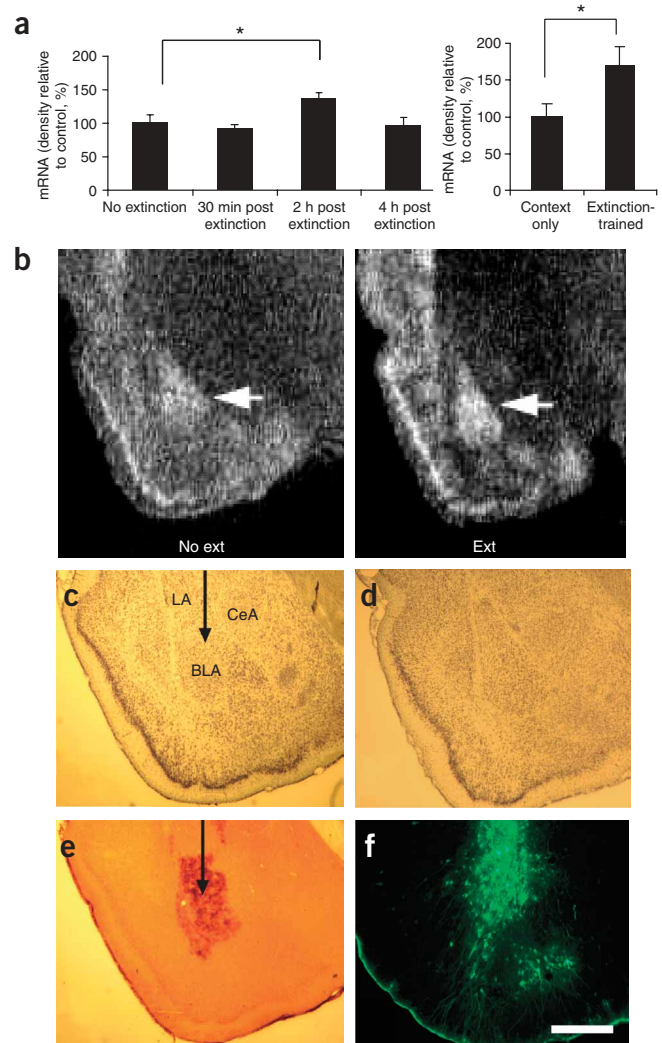
Figure 1 Bdnf mRNA expression and assessment of lentiviral gene expression within the BLA. (a) Regulation of Bdnf mRNA following extinction. In situ hybridization was used to assess the amount of Bdnf mRNA (exon V) present at three time points following extinction. n = 6 per group. At right, a replication experiment in which some rats underwent the same extinction protocol as on the left, whereas others were simply placed in the extinction context without light presentations. Both groups were killed 2 h after the exposure. n = 8 per group. (b) At the 2-h time point, significant increases in Bdnf mRNA were found within the basolateral amygdala (BLA, arrow), as shown with dark-field optics. (c,d) Histological examination of viral infection in the BLA following behavioral studies. No amygdala damage was seen following infection (visualized with cresyl violet staining). LA, lateral amygdala. CeA, central amygdala. (e) Expression of TrkB.t1 was assessed using immunocytochemistry (ICC) for a hemagglutinin (HA) epitope tag incorporated into the TrkB.t1 coding sequence. (f) GFP expression was directly assessed by visualizing tissue under an epifluorescence microscope. * P < 0.05 . Error bars represent s.e.m. Scale bar, 1 mm.
